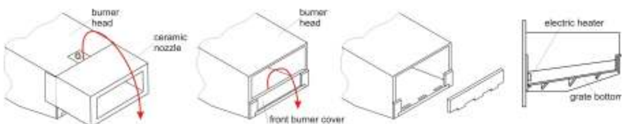
Removal of the front burner covers for easier cleaning and correct grate position
