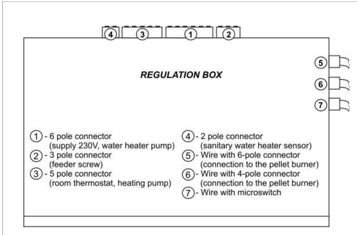
Figure: Connectors at the control unit box
